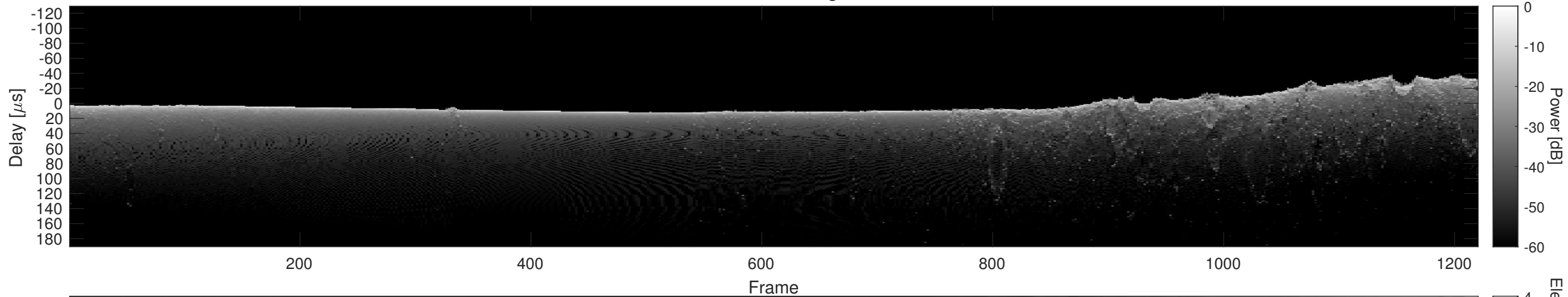
Orbit 7270, Cluttergram
