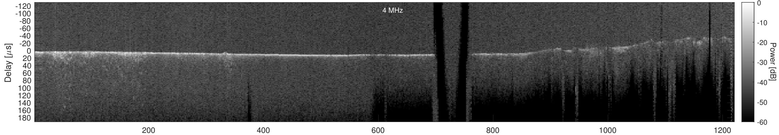
Orbit 7270, Cluttergram
