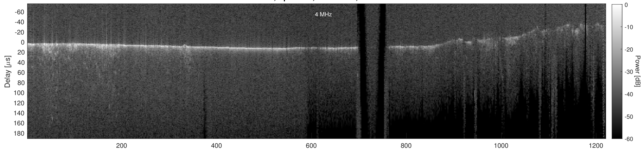
Orbit 7270, Cluttergram
