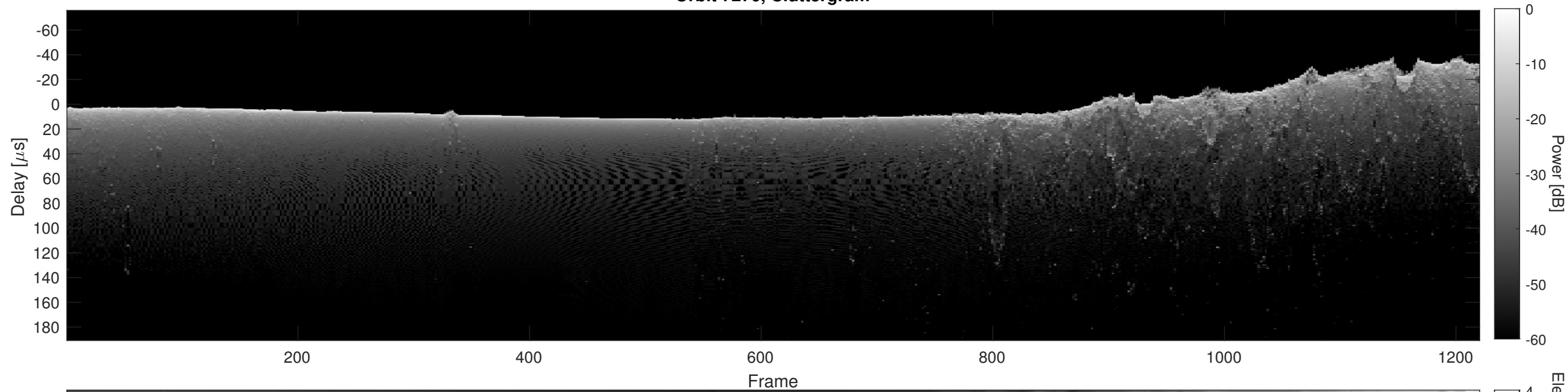
Orbit 7270, Cluttergram
