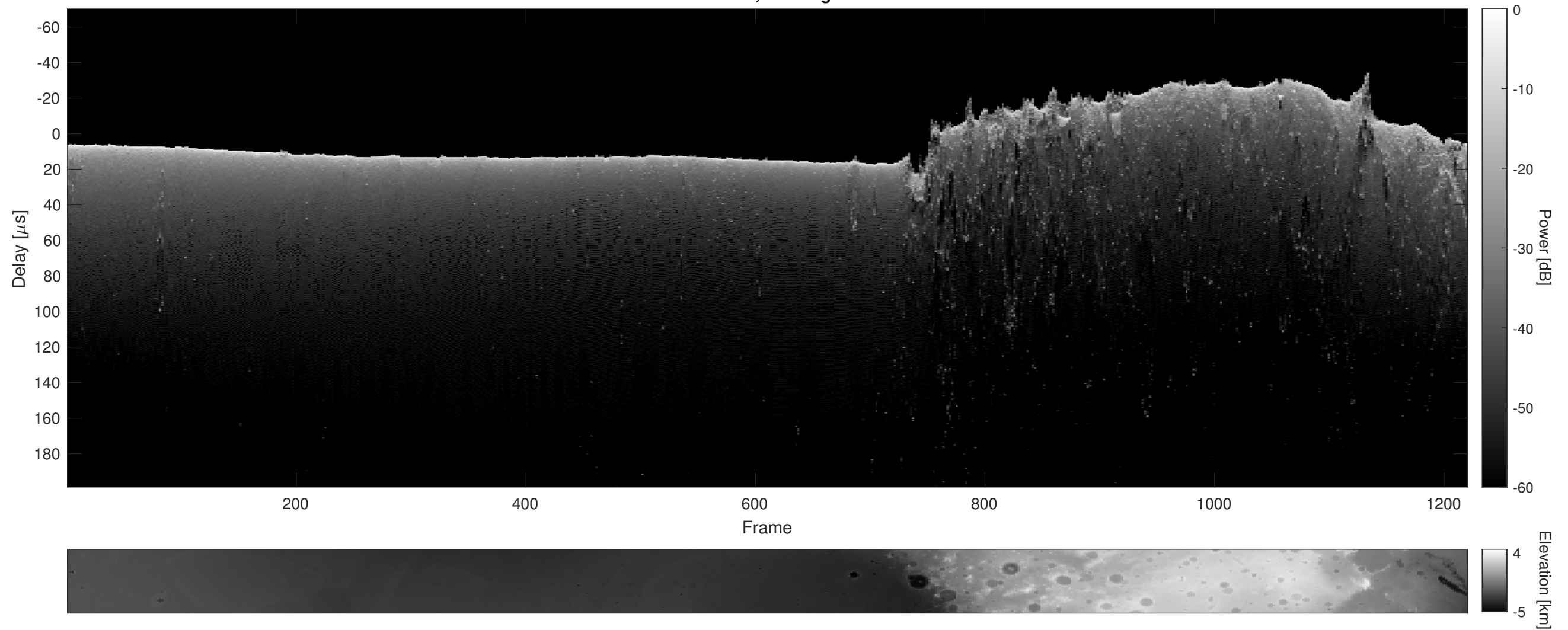
Orbit 7271, Cluttergram
