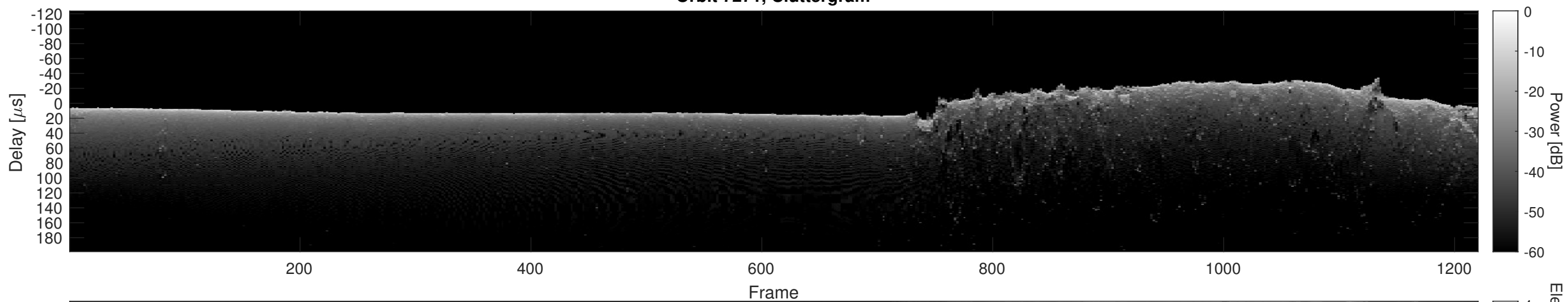
Orbit 7271, Cluttergram
