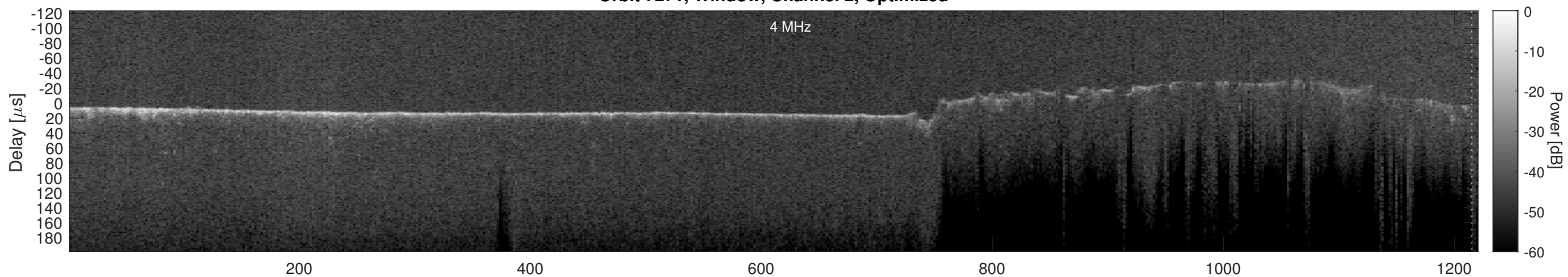
Orbit 7271, Cluttergram
