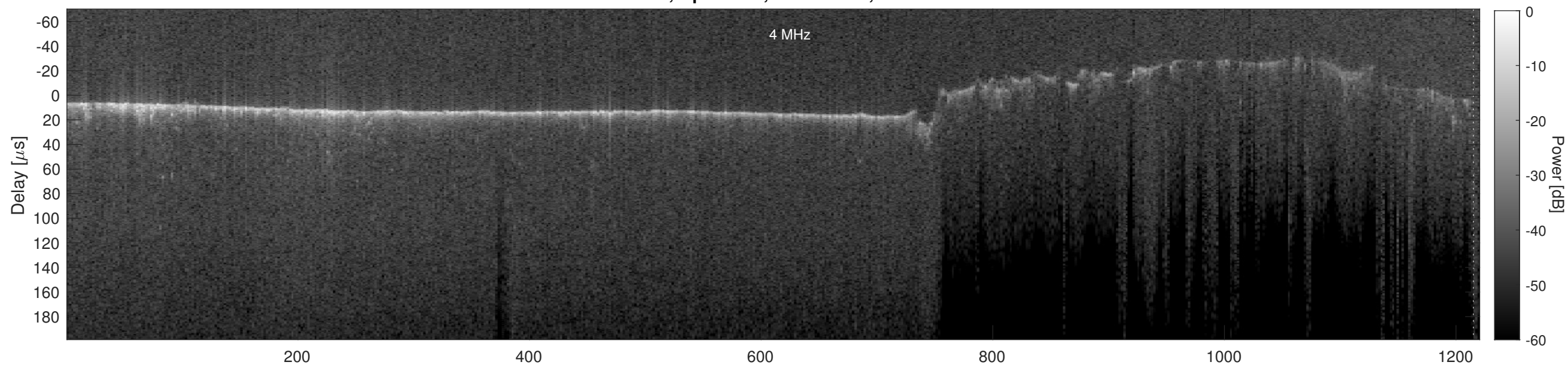
Orbit 7271, Cluttergram
