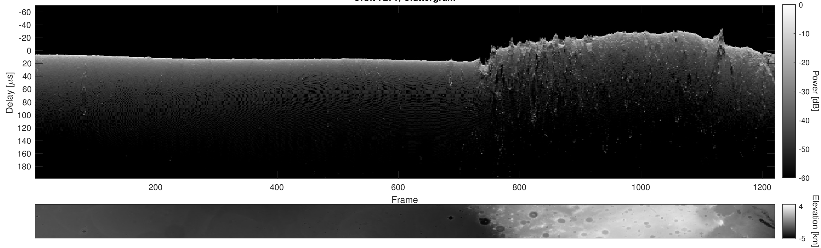
Orbit 7271, Cluttergram
