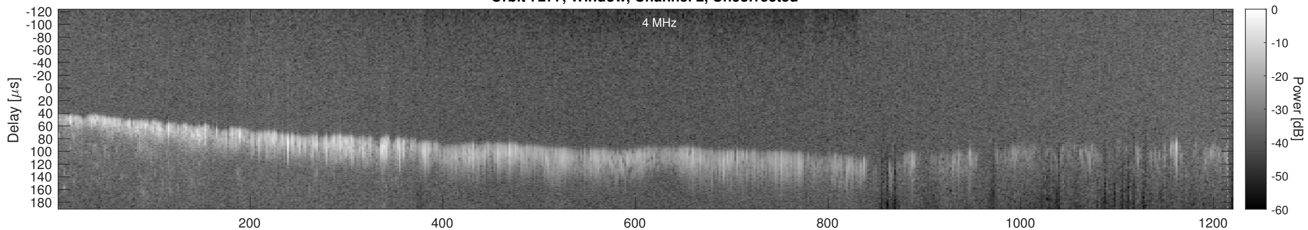
Orbit 7277, Window, Channel 2, Chapman
