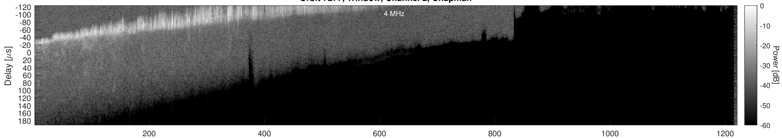
Orbit 7277, Window, Channel 2, Optimized
