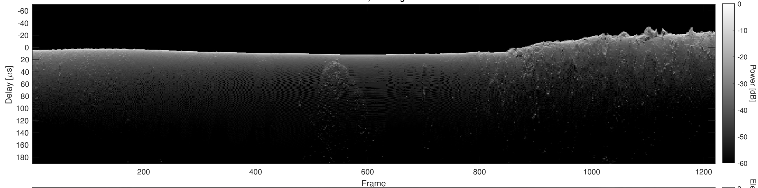
Orbit 7277, Cluttergram
