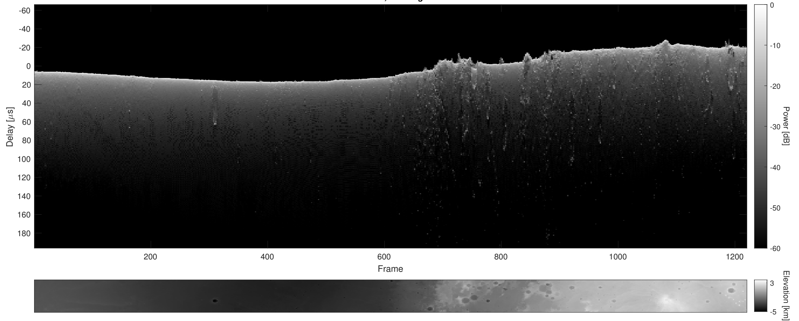
Orbit 7278, Cluttergram
