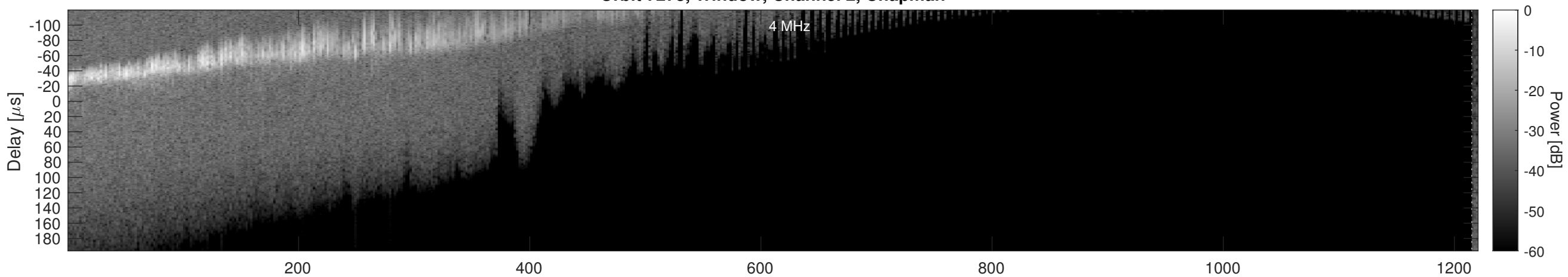
Orbit 7278, Window, Channel 2, Optimized
