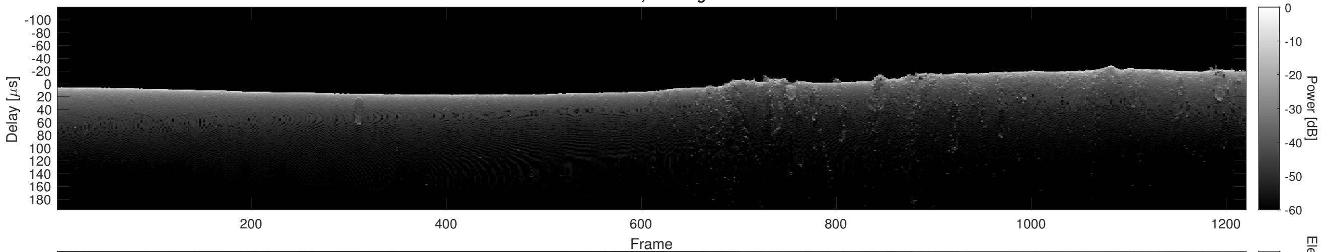
Orbit 7278, Cluttergram
