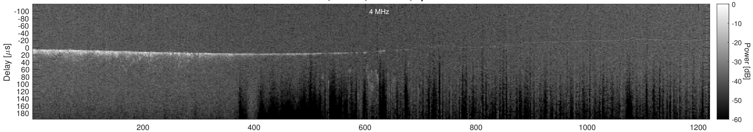
Orbit 7278, Cluttergram
