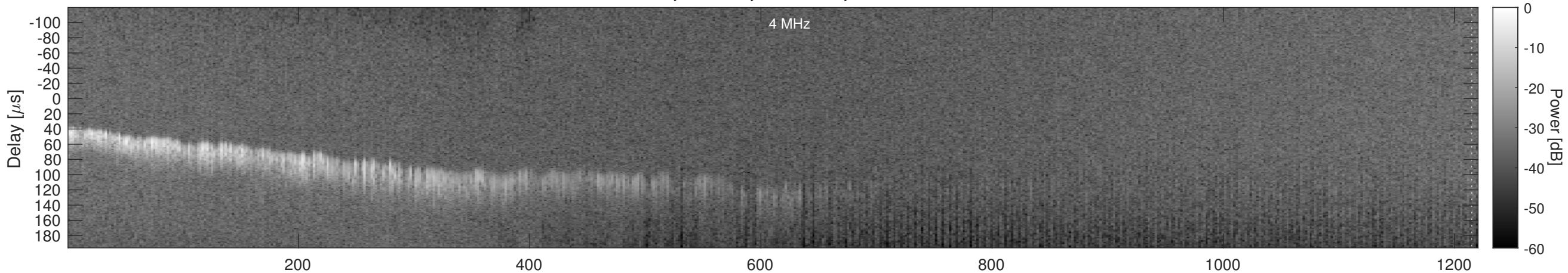
Orbit 7278, Window, Channel 2, Chapman
