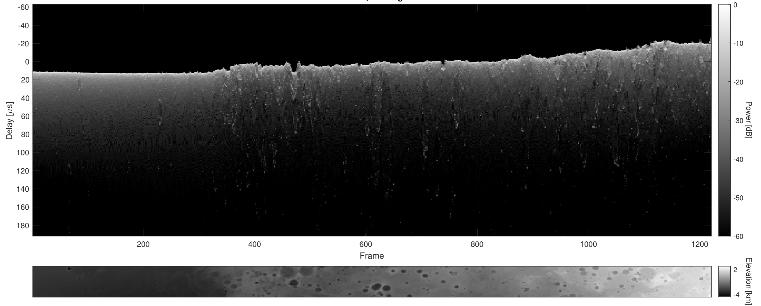
Orbit 7279, Cluttergram
