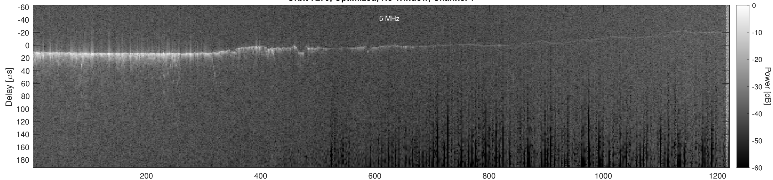
Orbit 7279, Optimized, No Window, Channel 2
