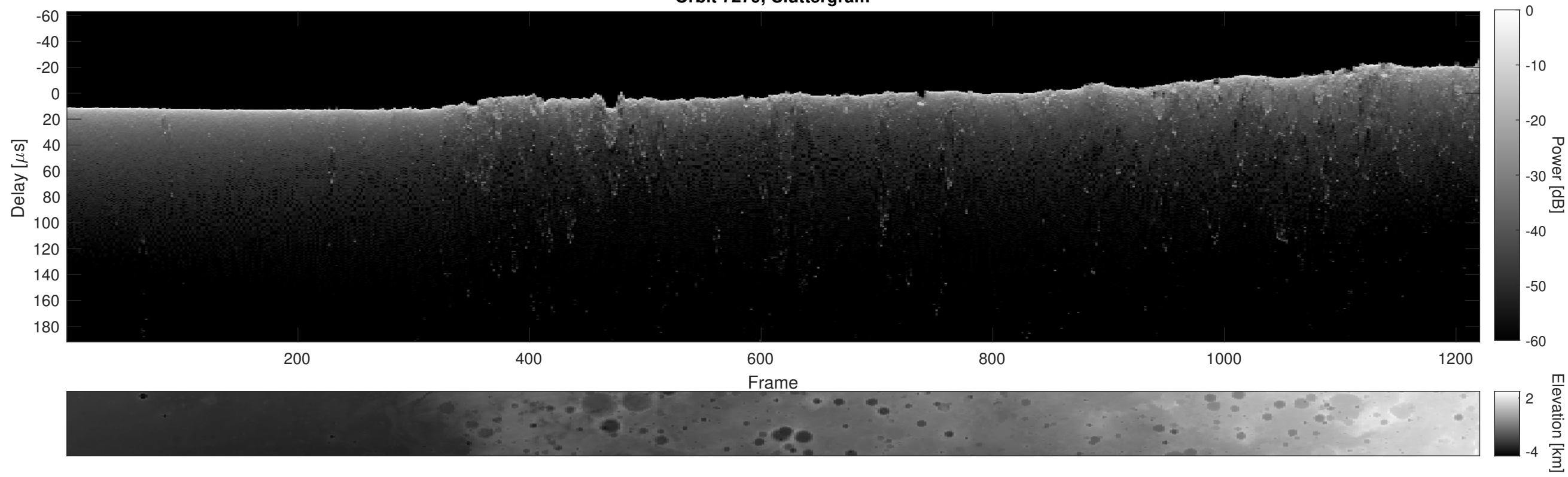
Orbit 7279, Cluttergram
