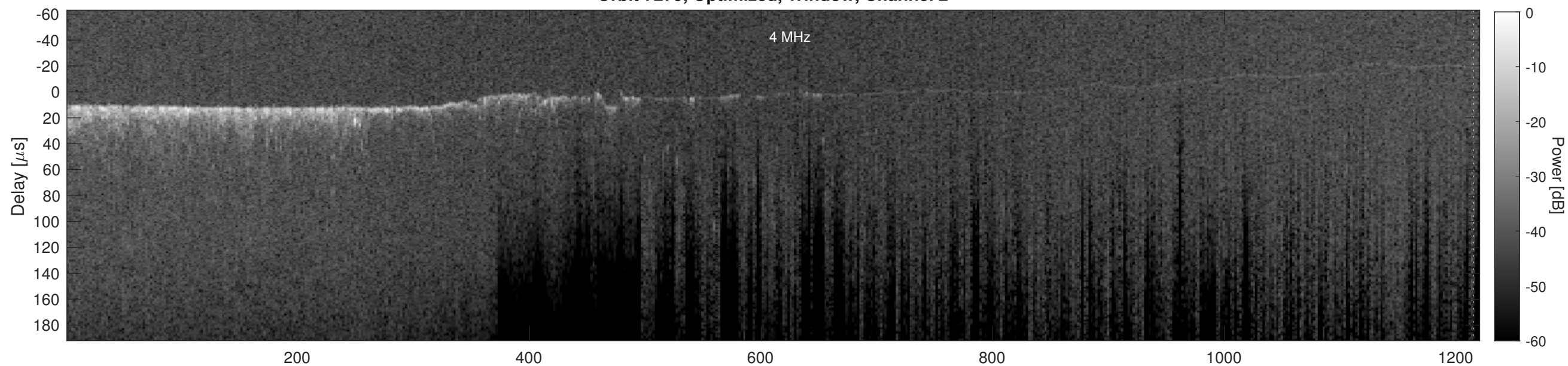
Orbit 7279, Cluttergram
