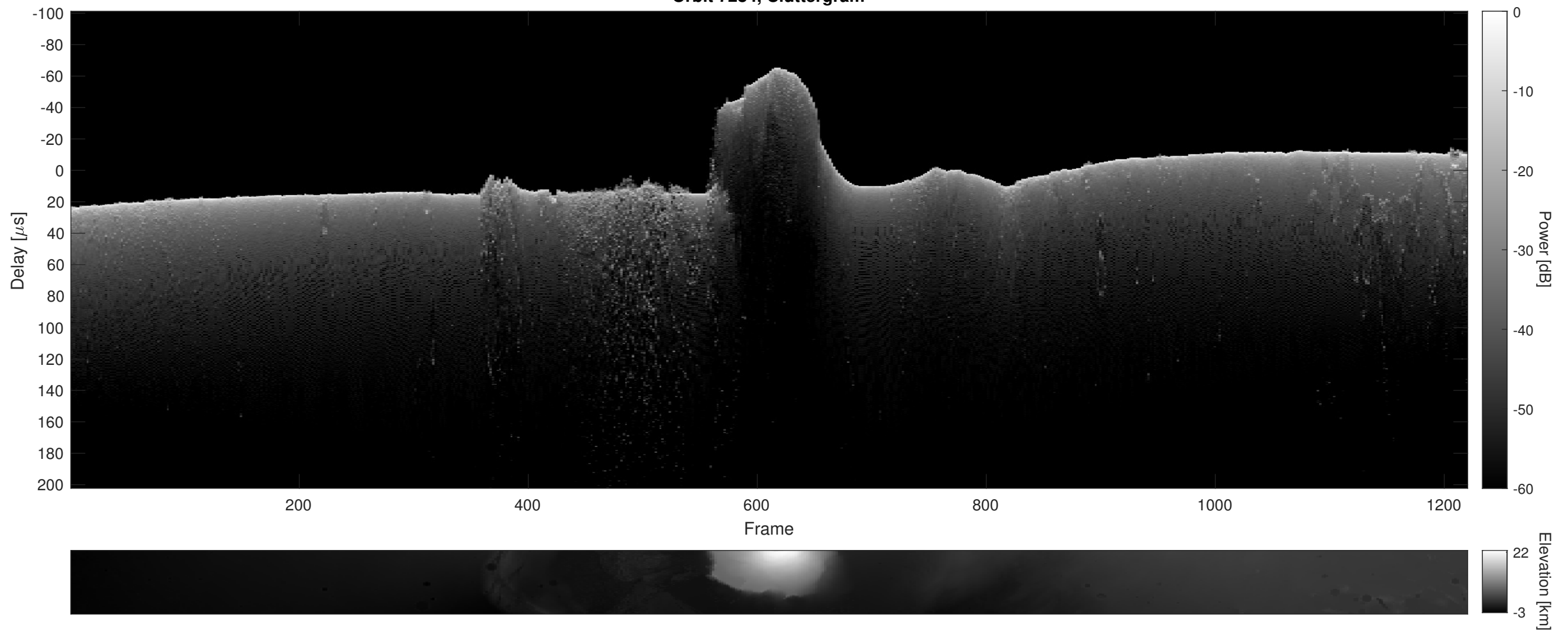
Orbit 7284, Cluttergram
