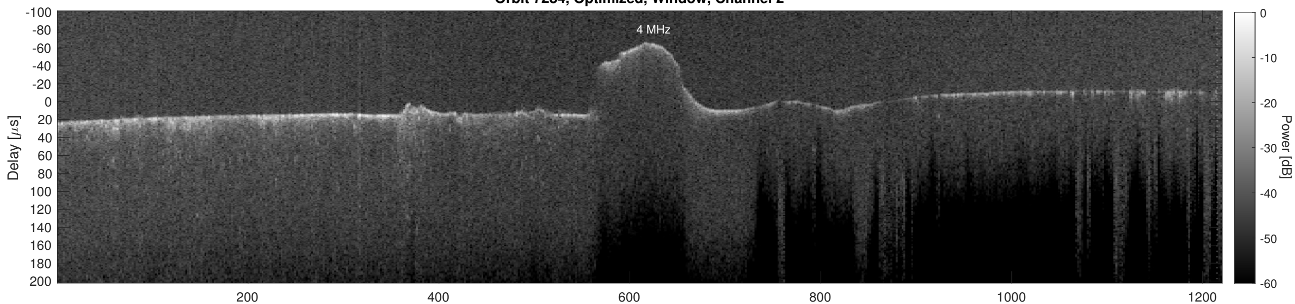
Orbit 7284, Cluttergram
