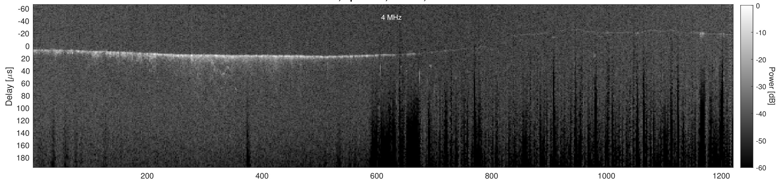
Orbit 7285, Cluttergram
