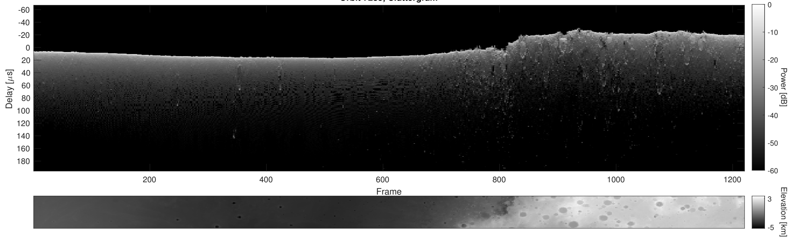
Orbit 7285, Cluttergram
