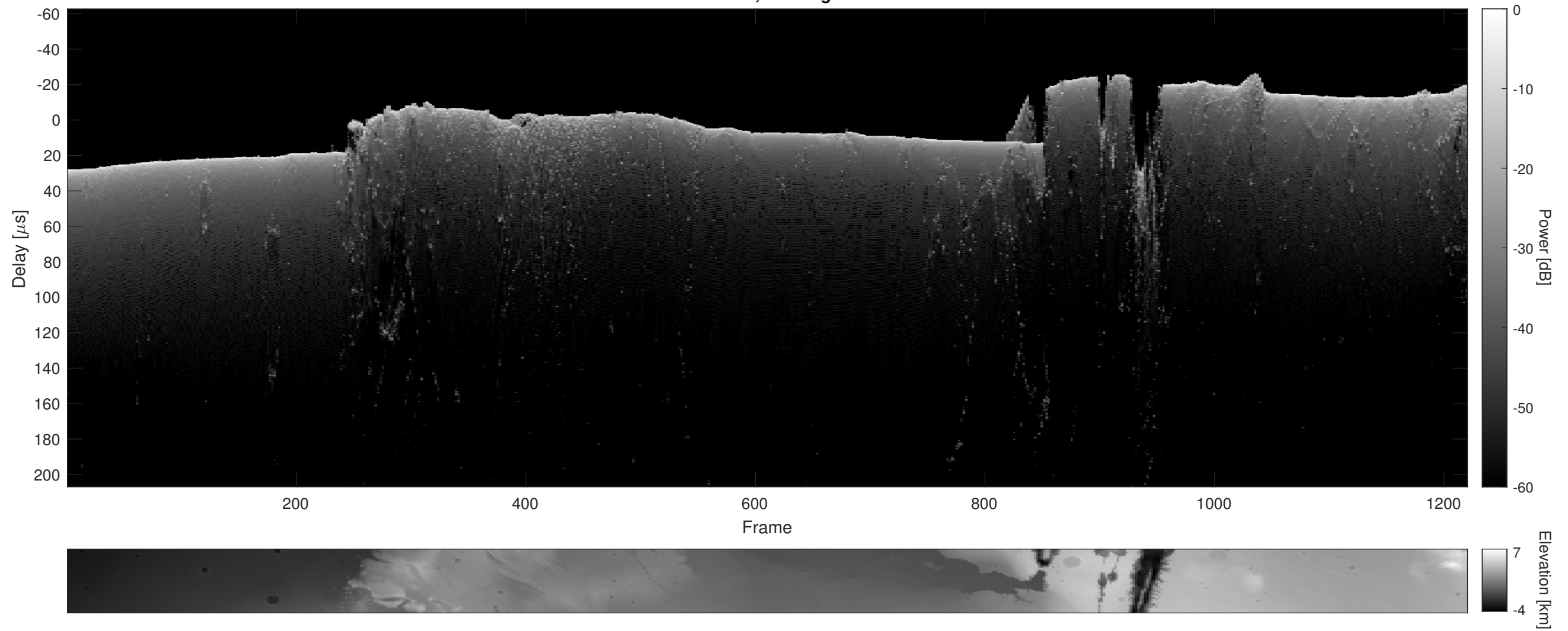
Orbit 7287, Cluttergram
