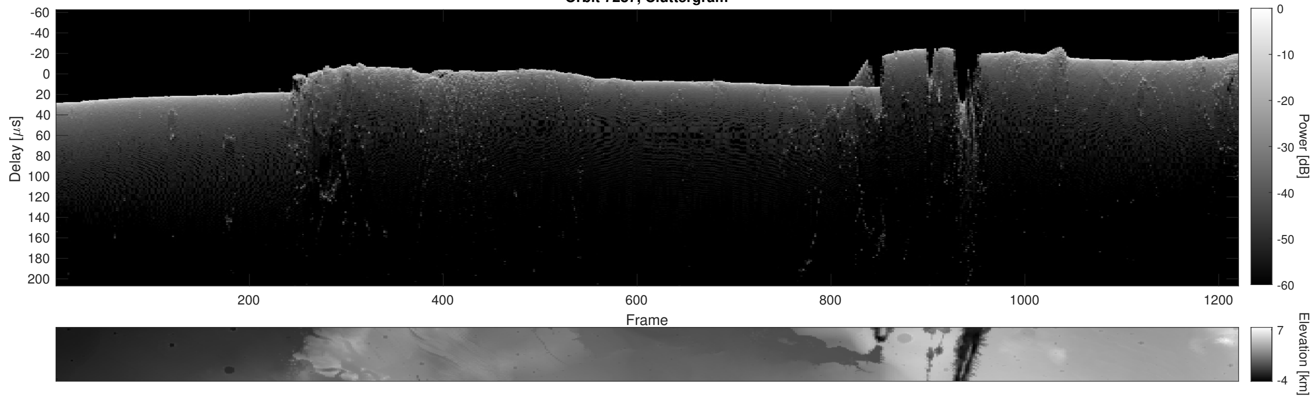
Orbit 7287, Cluttergram
