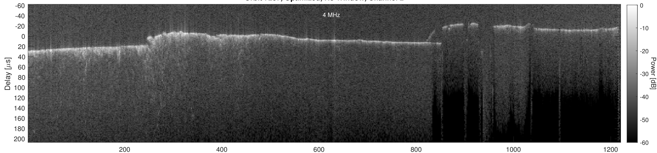
Orbit 7287, Cluttergram
