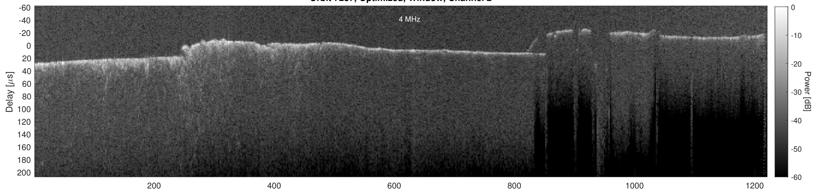
Orbit 7287, Cluttergram
