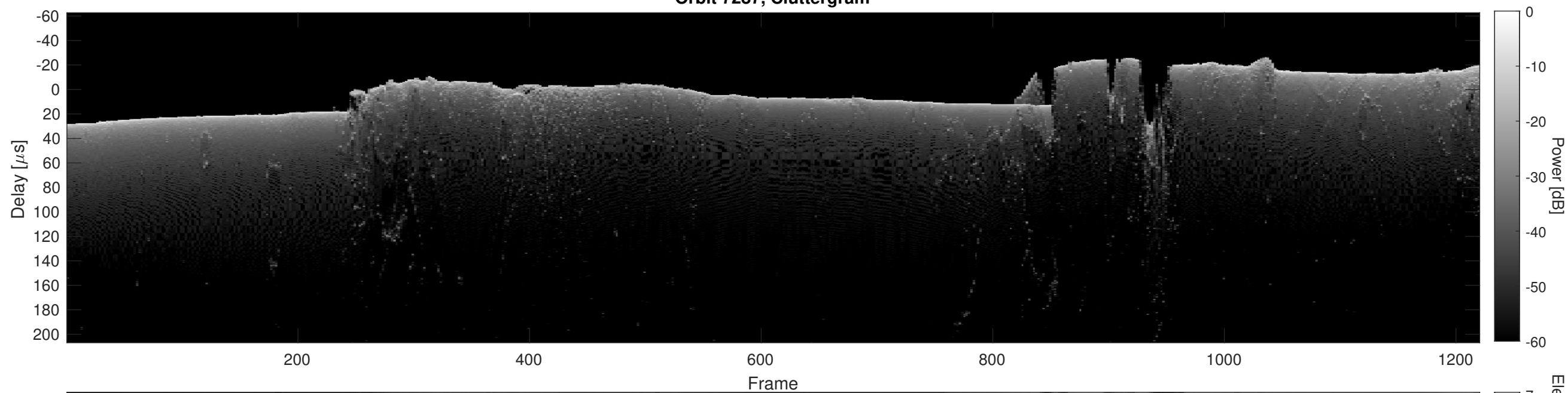
Orbit 7287, Cluttergram
