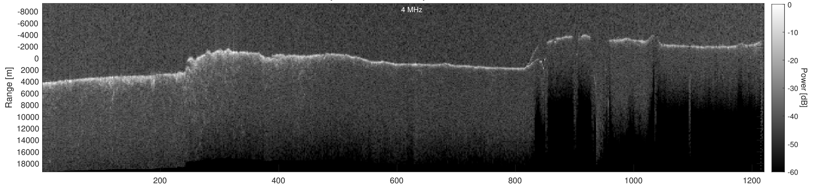
Orbit 7287, Depth-Corrected Cluttergram
