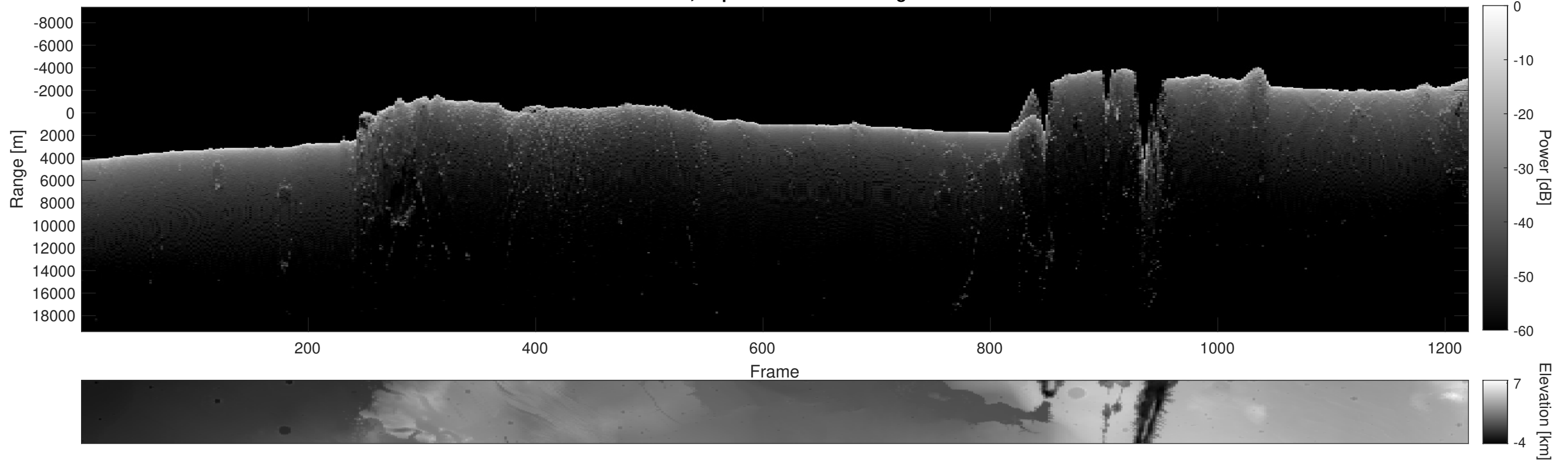
Orbit 7287, Depth-Corrected Cluttergram
