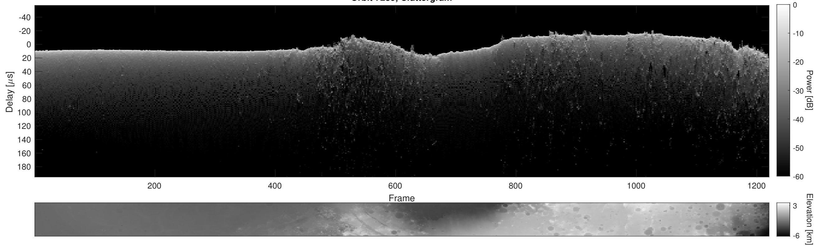
Orbit 7289, Cluttergram
