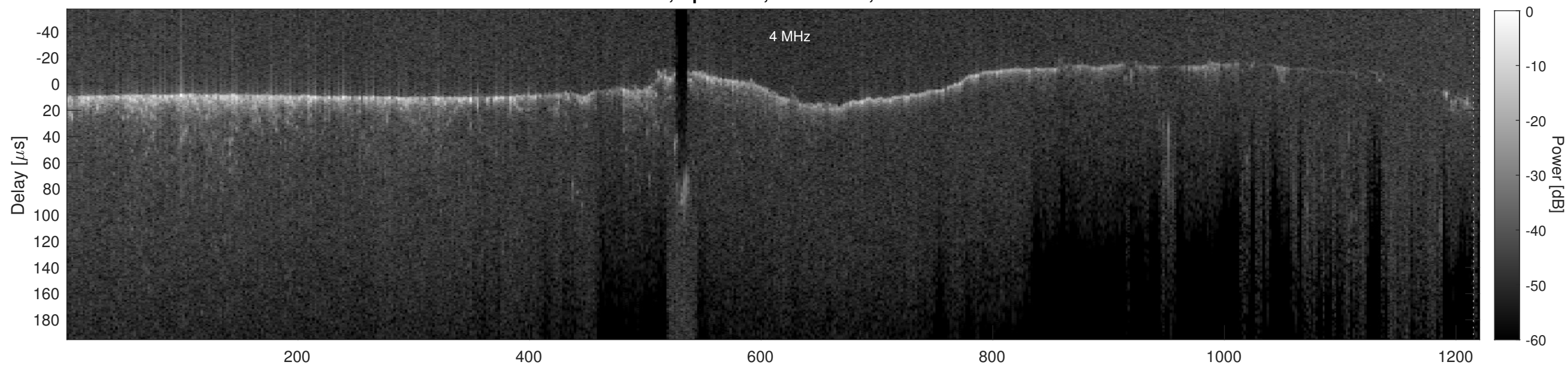
Orbit 7289, Cluttergram
