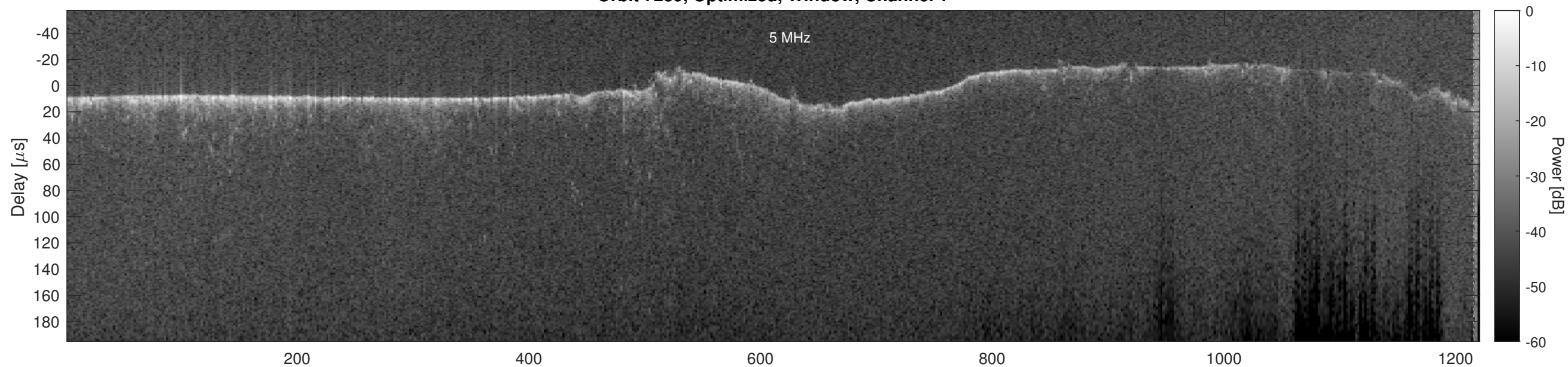
Orbit 7289, Optimized, Window, Channel 2
