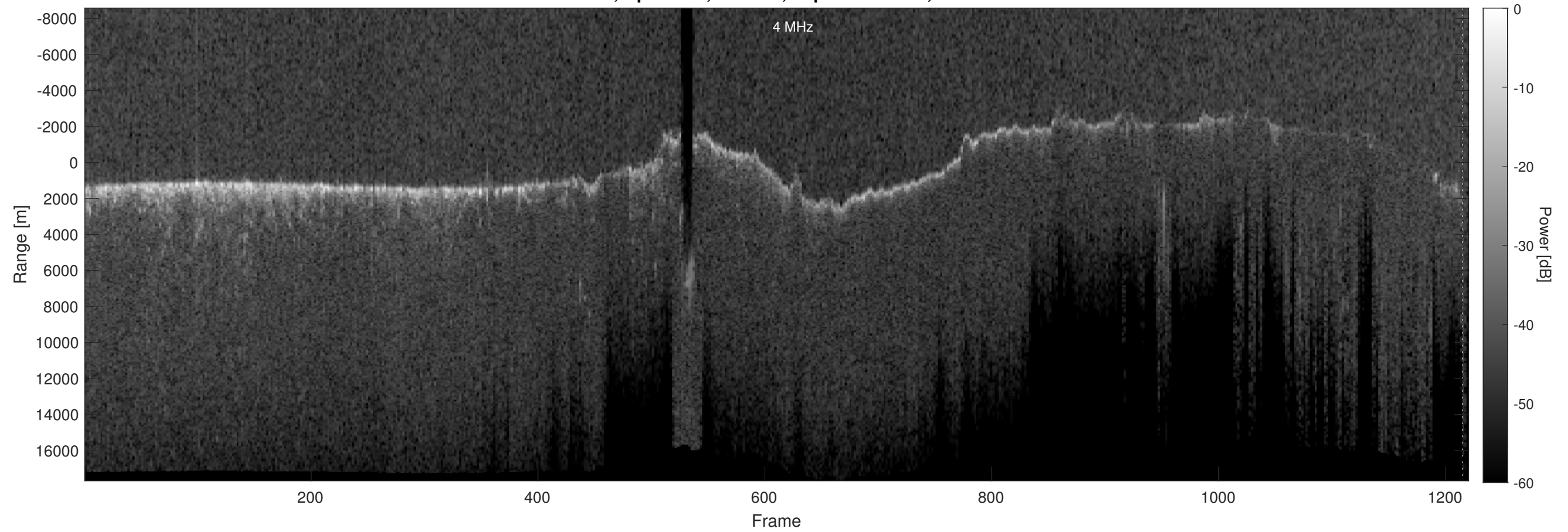
Orbit 7289, Optimized, Window, Depth-Corrected, Channel 2
