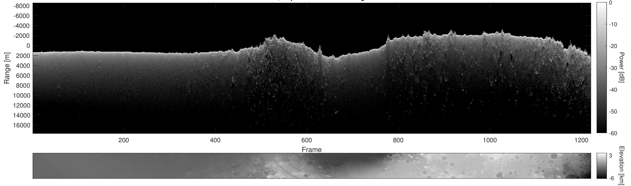
Orbit 7289, Depth-Corrected Cluttergram
