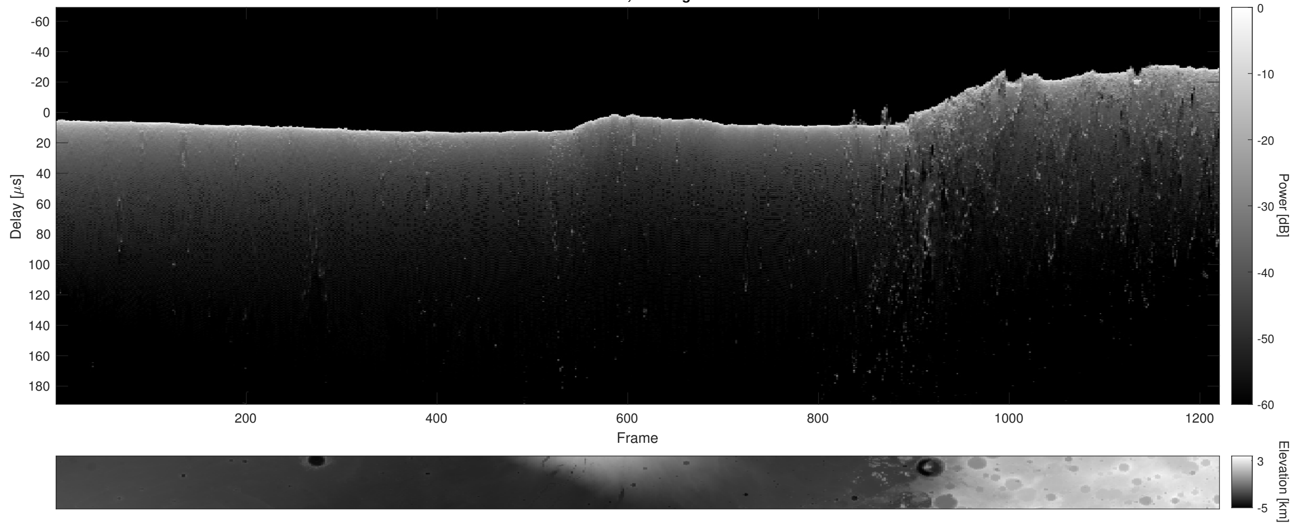
Orbit 7292, Cluttergram
