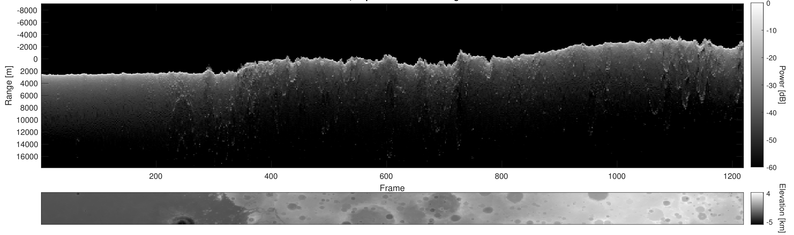
Orbit 7293, Depth-Corrected Cluttergram
