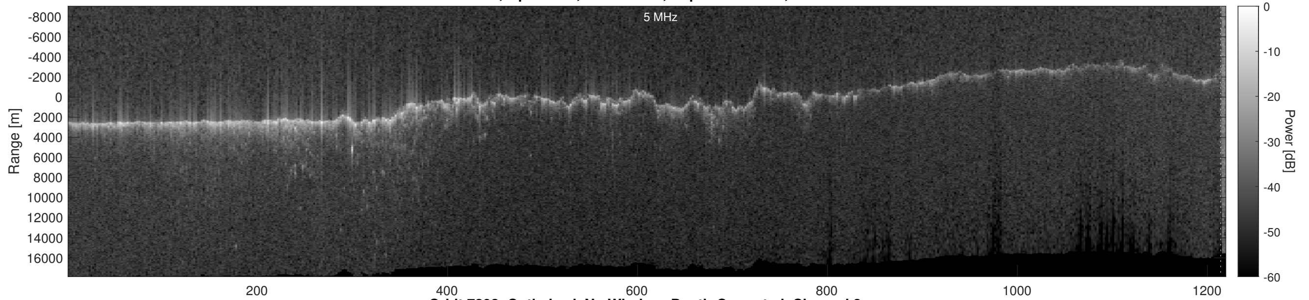
Orbit 7293, Optimized, No Window, Depth-Corrected, Channel 2
