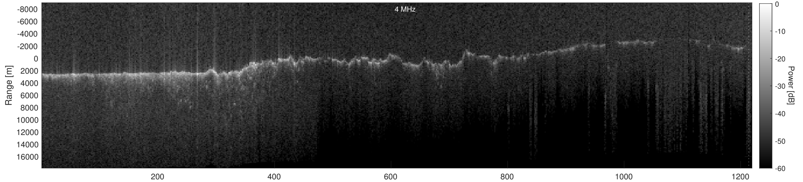
Orbit 7293, Depth-Corrected Cluttergram
