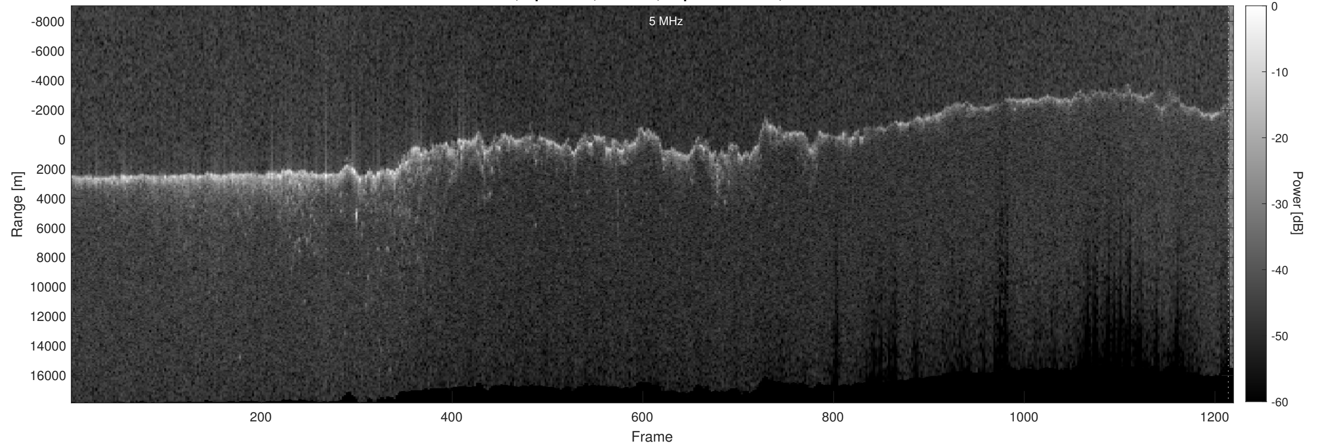
Orbit 7293, Optimized, Window, Depth-Corrected, Channel 2
