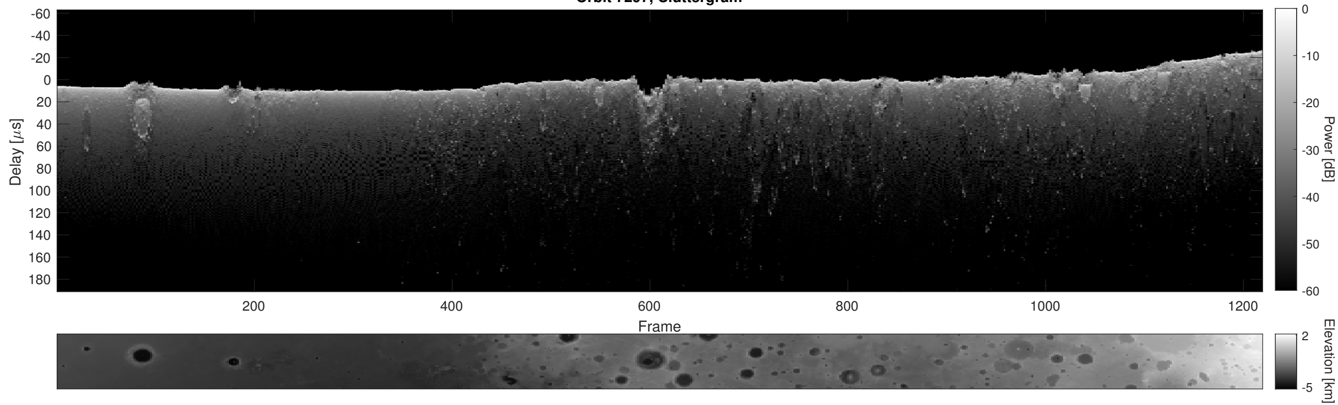
Orbit 7297, Cluttergram
