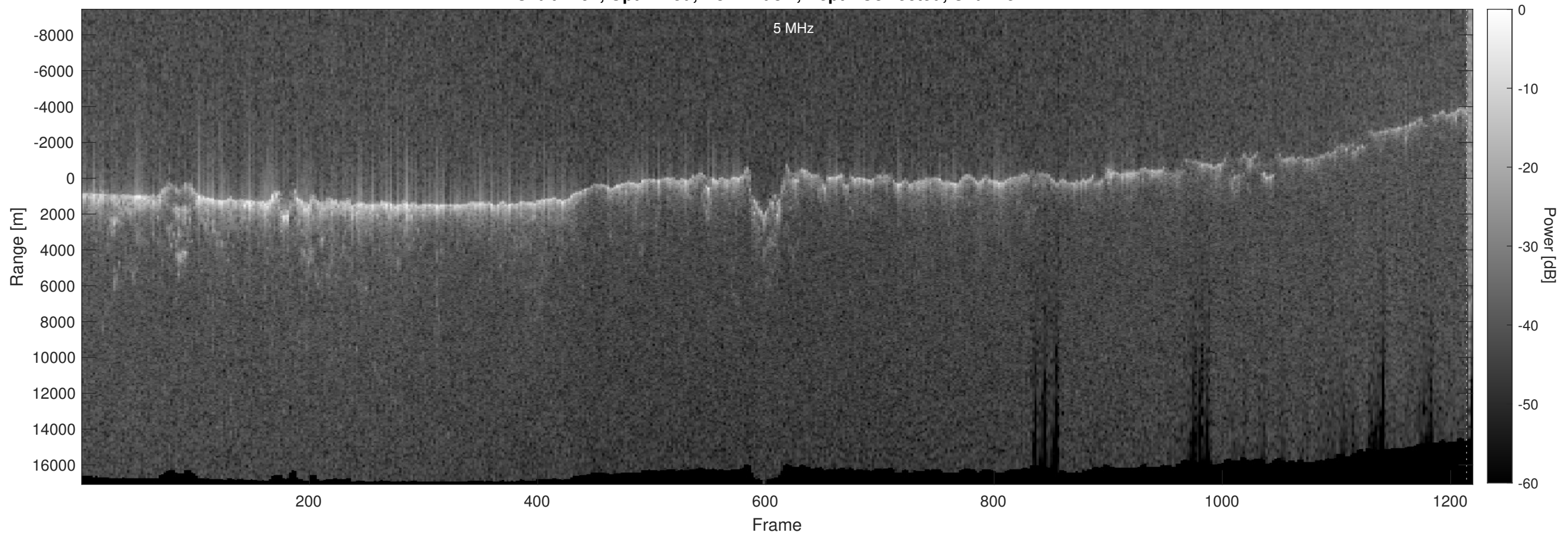
Orbit 7297, Optimized, No Window, Depth-Corrected, Channel 2
