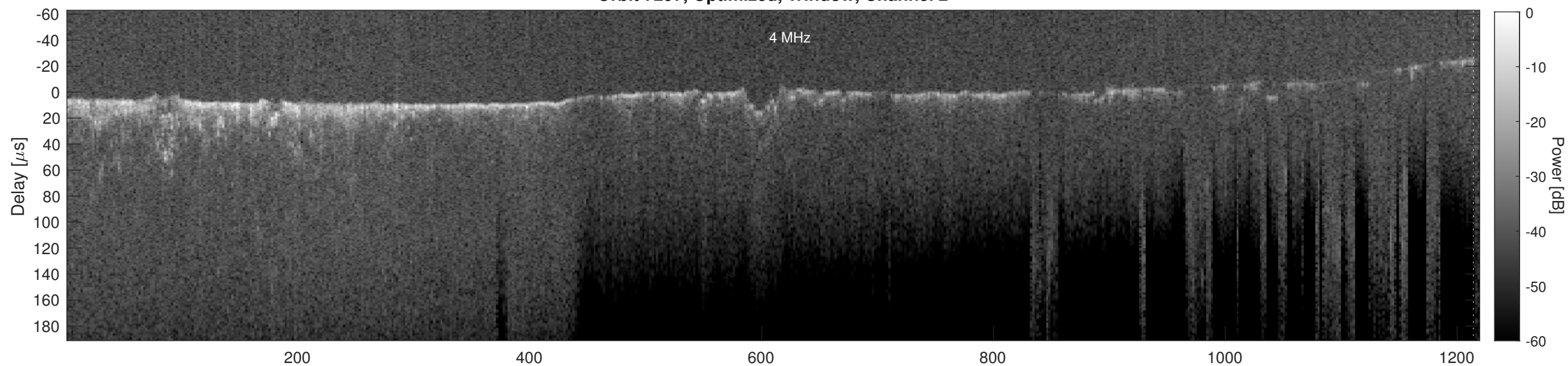
Orbit 7297, Cluttergram
