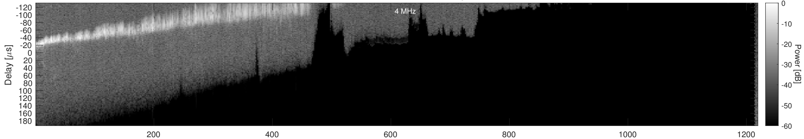
Orbit 7299, Window, Channel 2, Optimized
