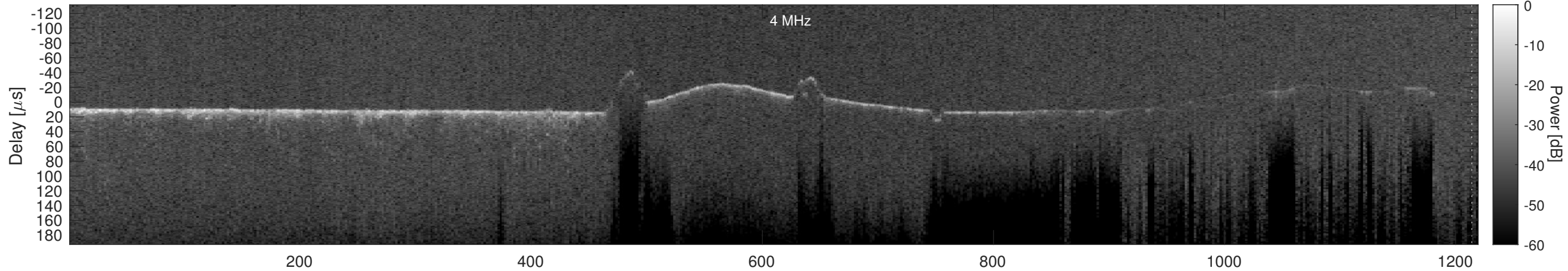
Orbit 7299, Cluttergram
