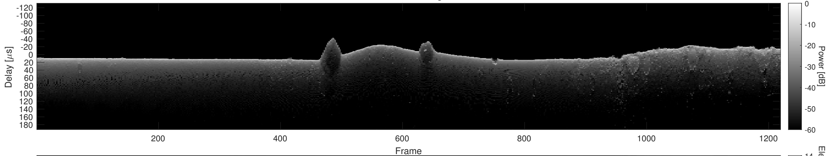
Orbit 7299, Cluttergram
