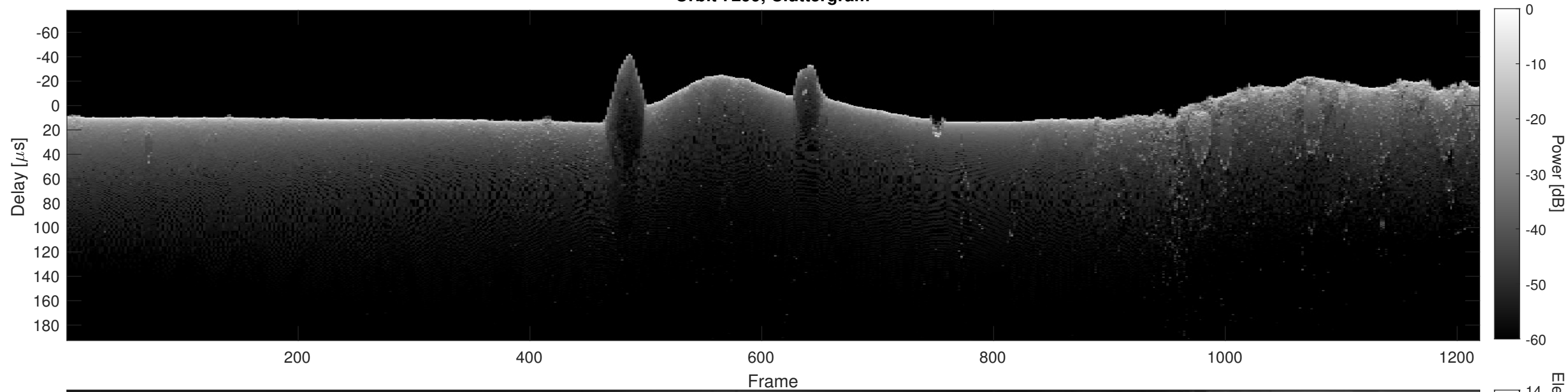
Orbit 7299, Cluttergram
