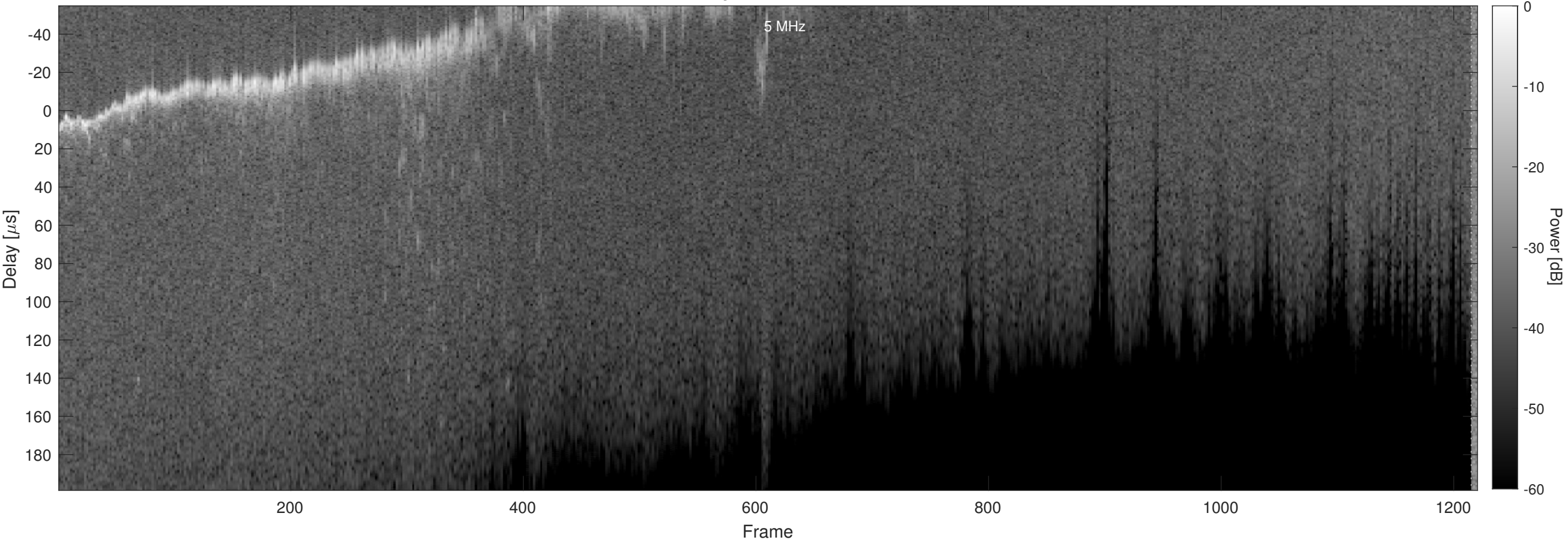
Orbit 7300, Chapman, Window, Channel 2
