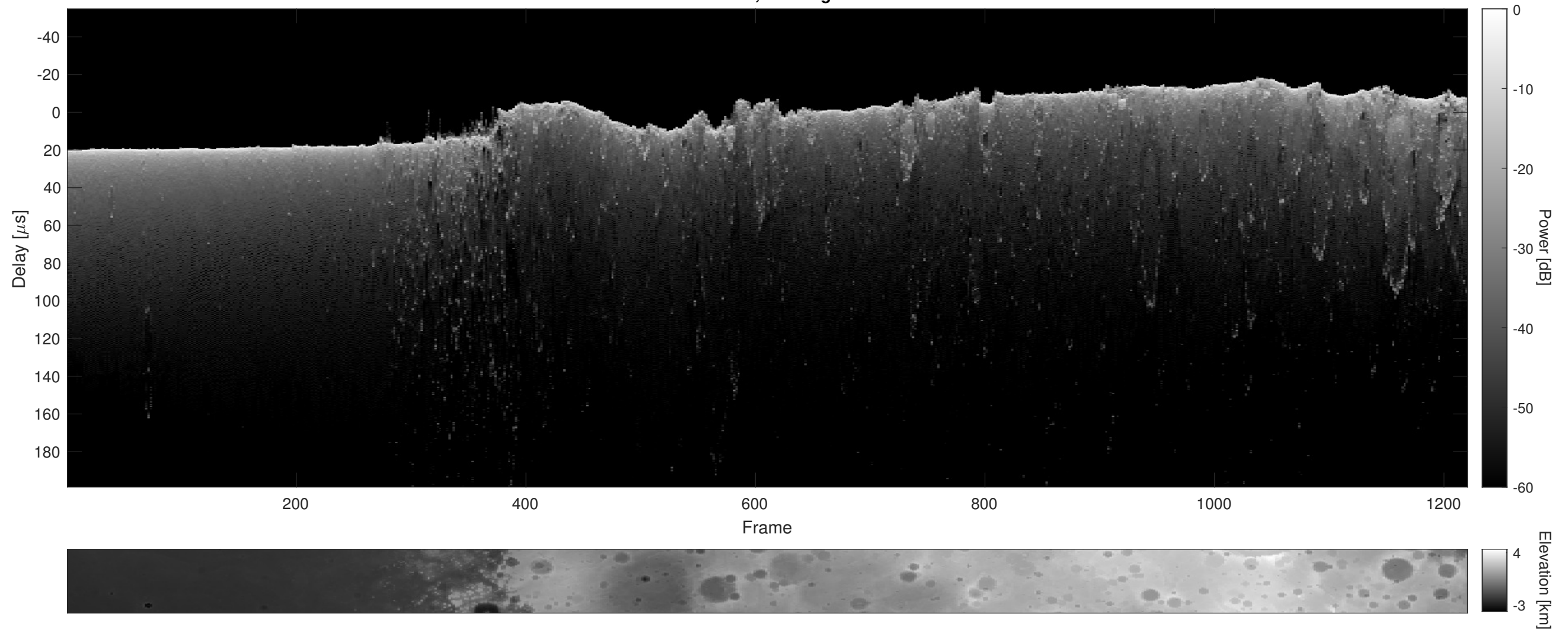
Orbit 7300, Cluttergram
