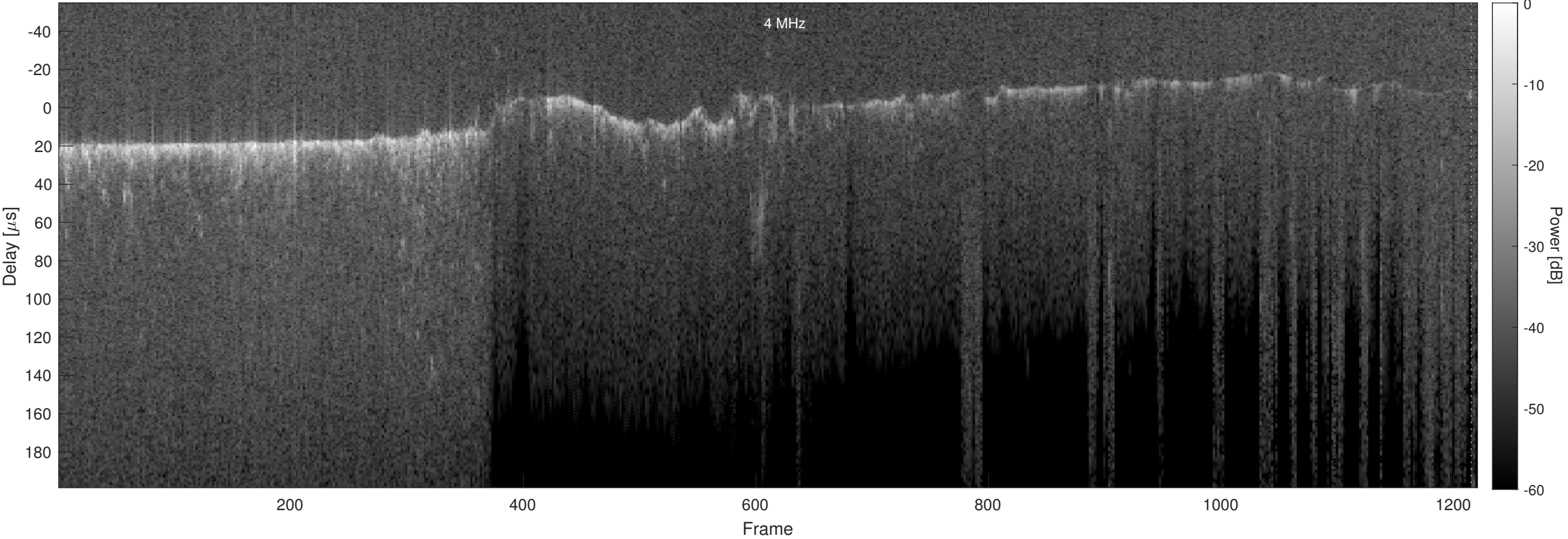
Orbit 7300, Optimized, No Window, Channel 2
