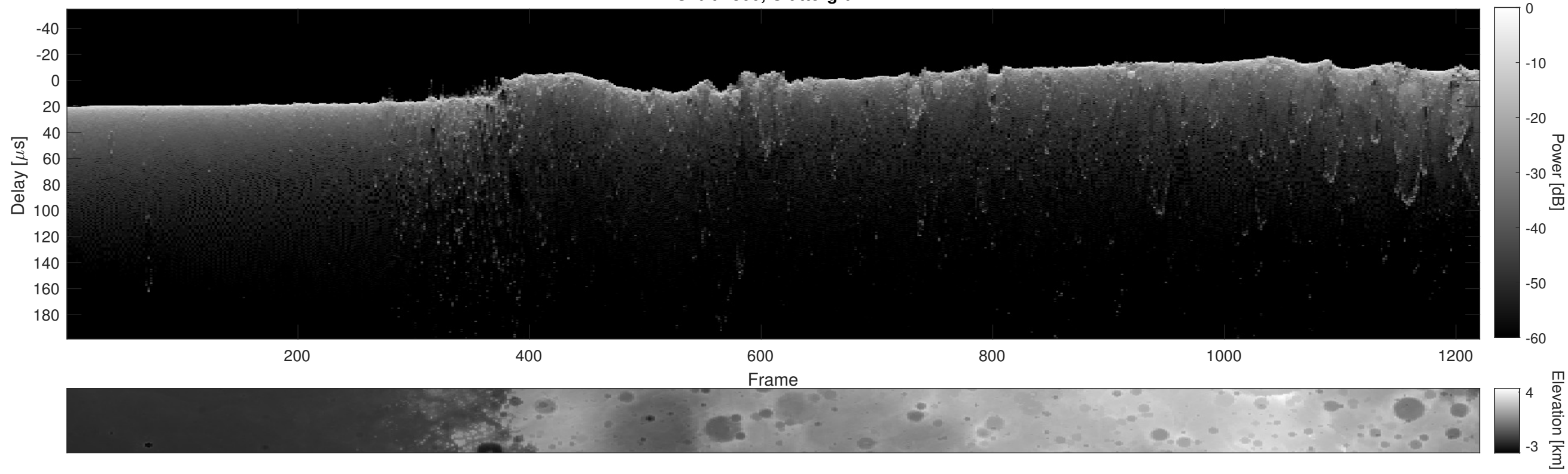
Orbit 7300, Cluttergram
