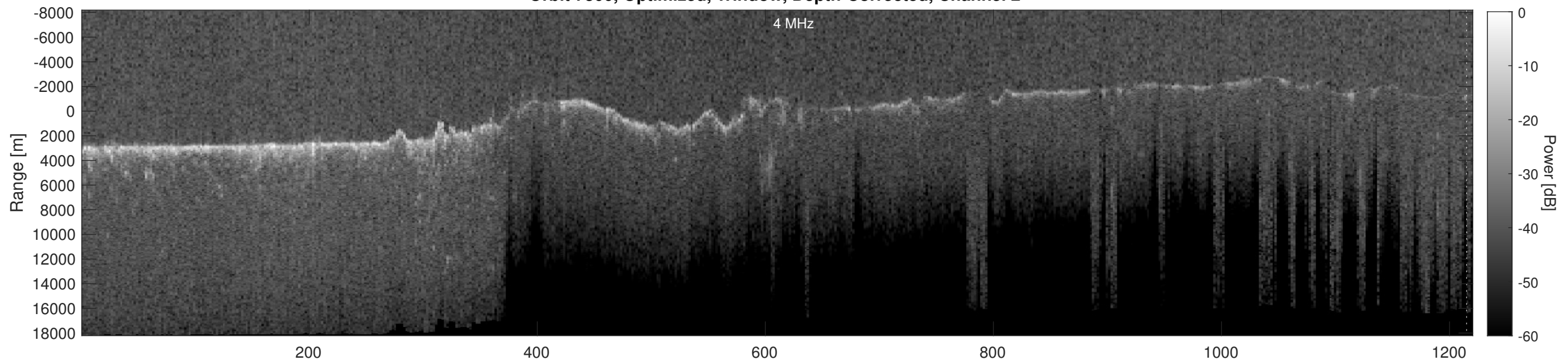
Orbit 7300, Depth-Corrected Cluttergram
