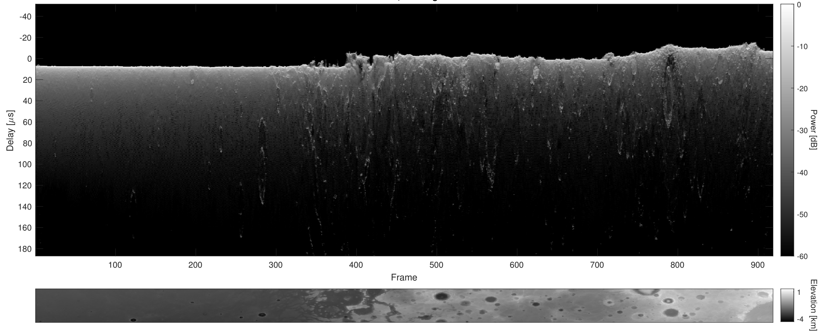
Orbit 7311, Cluttergram
