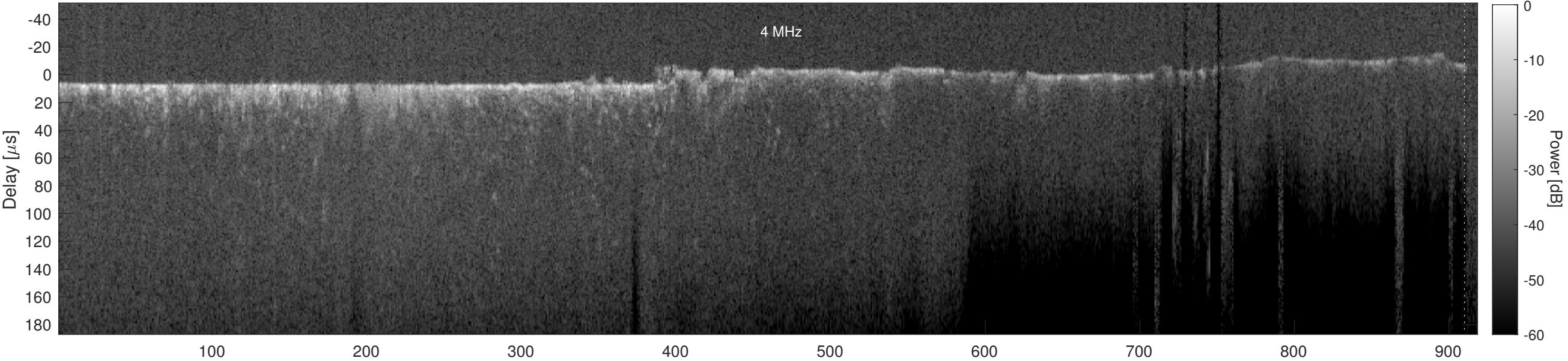
Orbit 7311, Cluttergram
