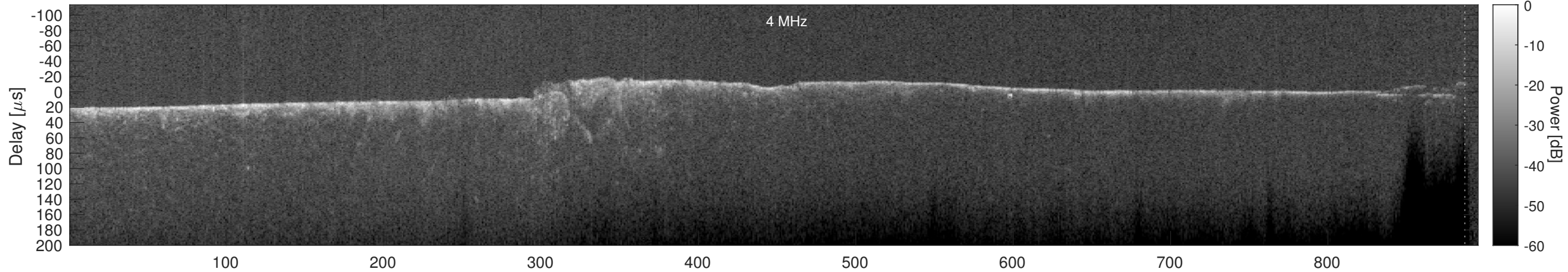
Orbit 7312, Cluttergram
