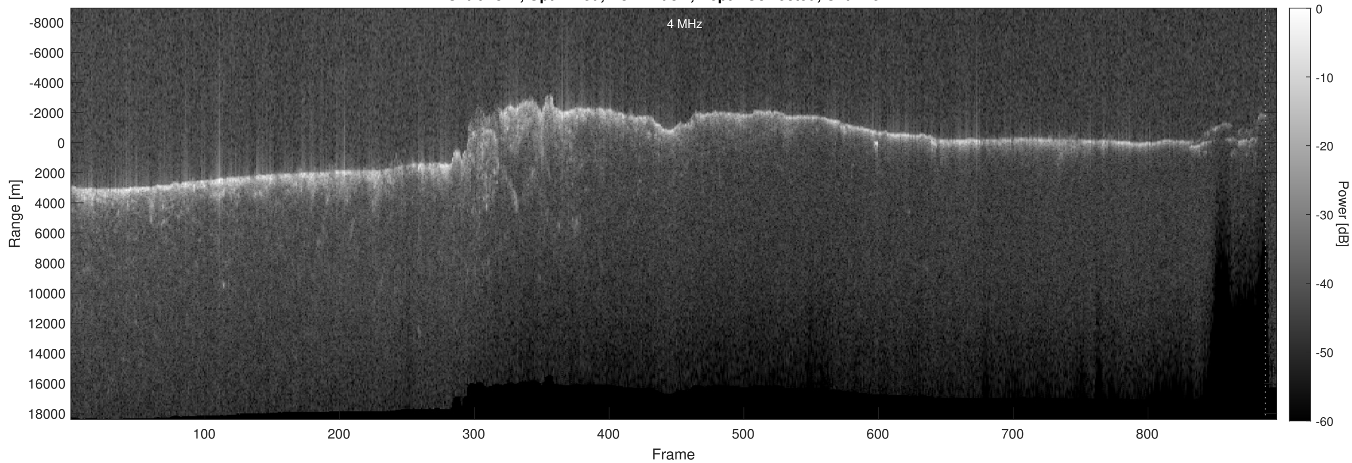
Orbit 7312, Optimized, No Window, Depth-Corrected, Channel 2
