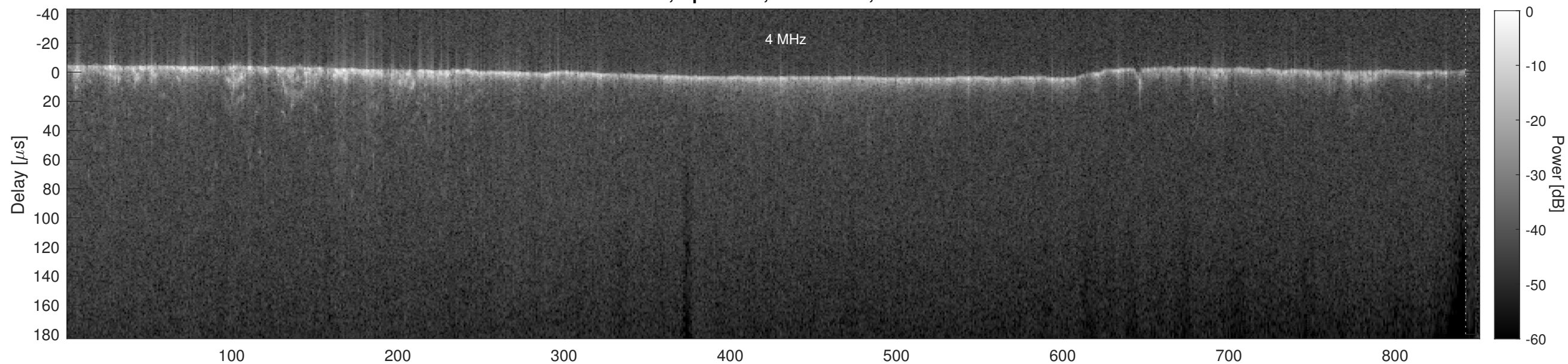
Orbit 7317, Cluttergram
