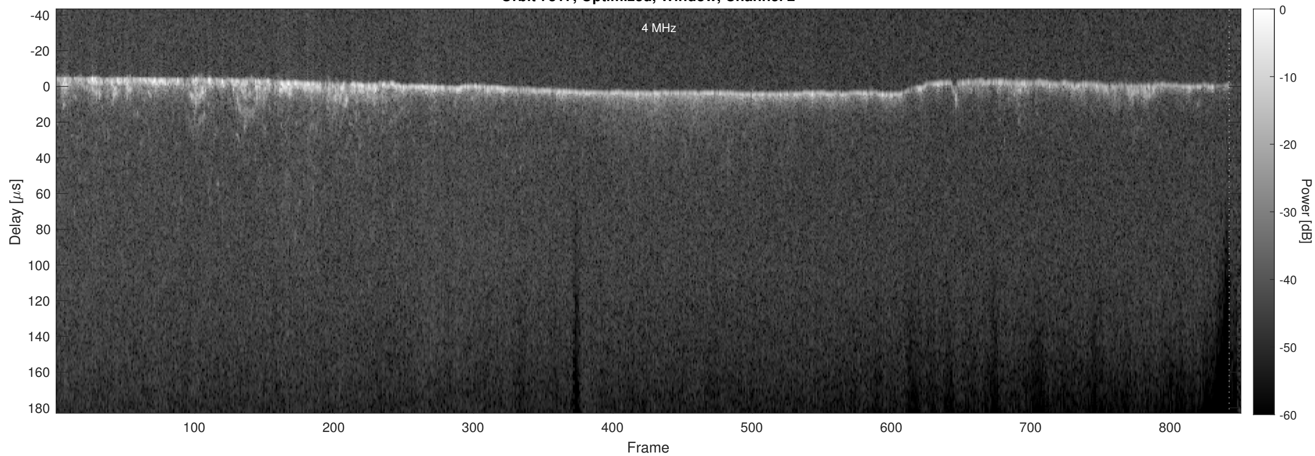
Orbit 7317, Optimized, Window, Channel 2
