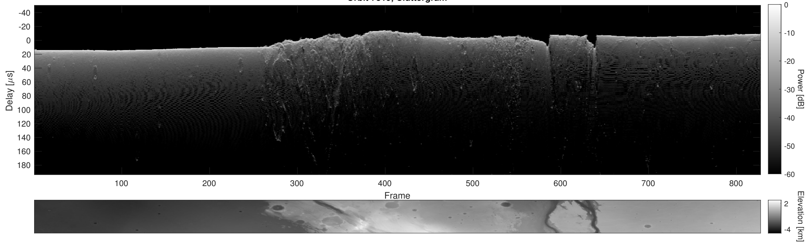
Orbit 7319, Cluttergram
