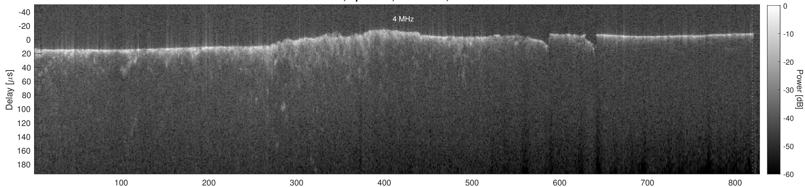
Orbit 7319, Cluttergram
