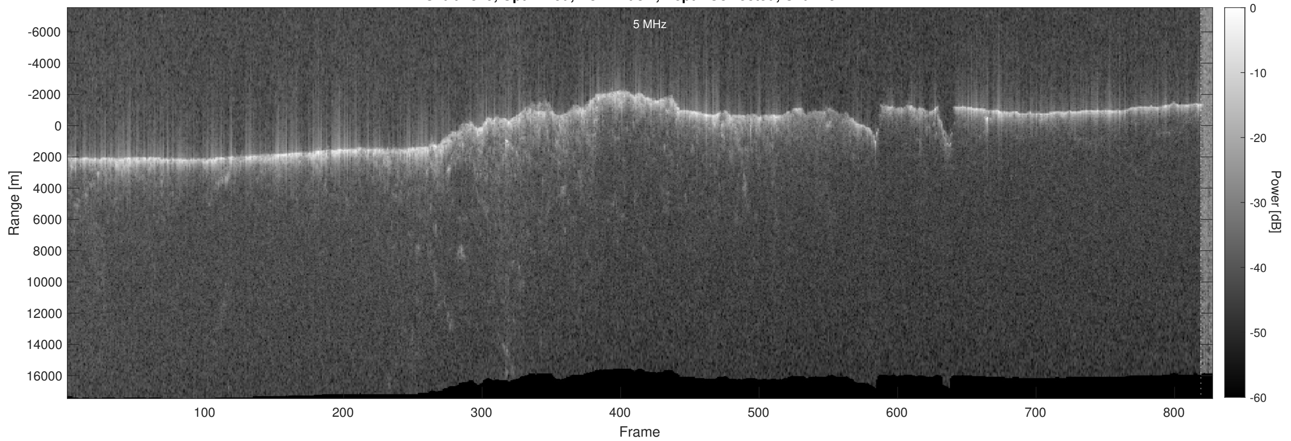
Orbit 7319, Optimized, No Window, Depth-Corrected, Channel 2
