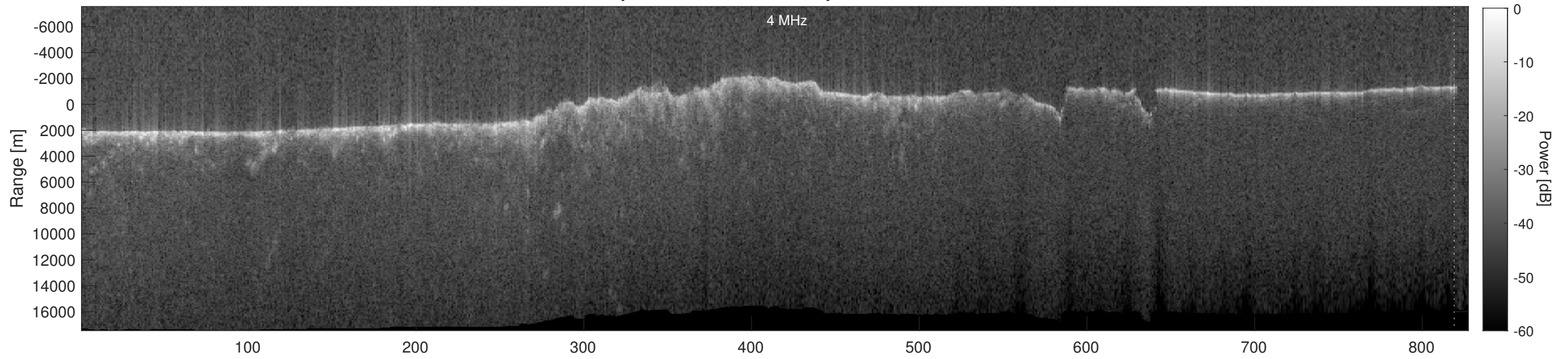
Orbit 7319, Depth-Corrected Cluttergram
