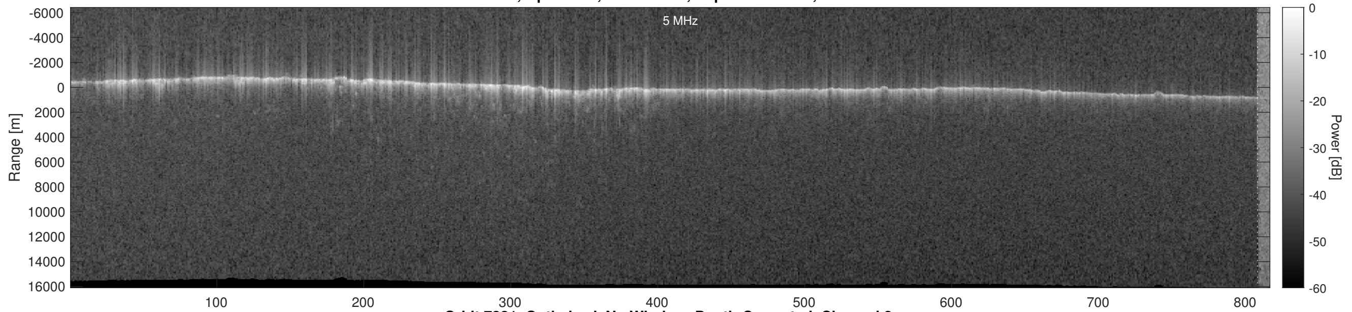
Orbit 7321, Optimized, No Window, Depth-Corrected, Channel 2
