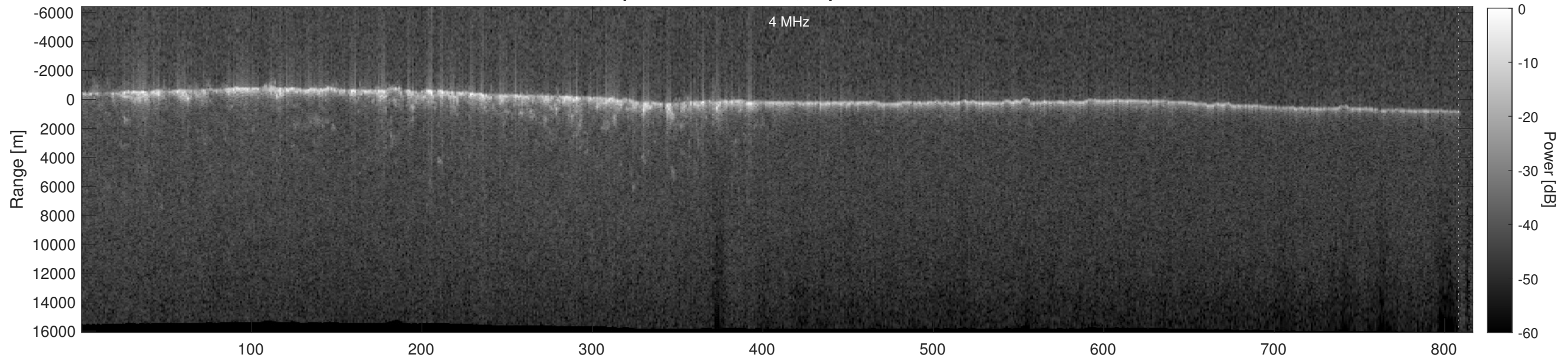
Orbit 7321, Depth-Corrected Cluttergram
