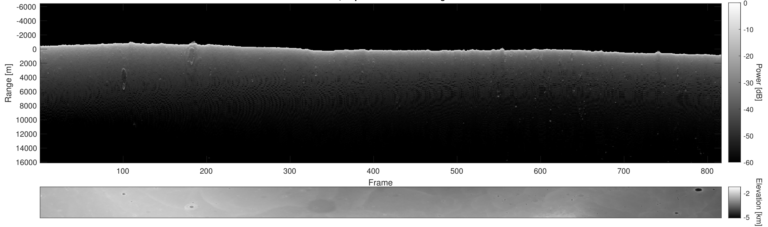
Orbit 7321, Depth-Corrected Cluttergram
