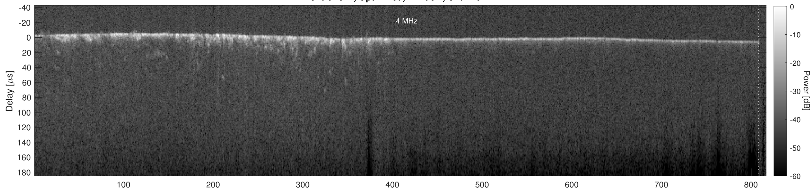
Orbit 7321, Cluttergram
