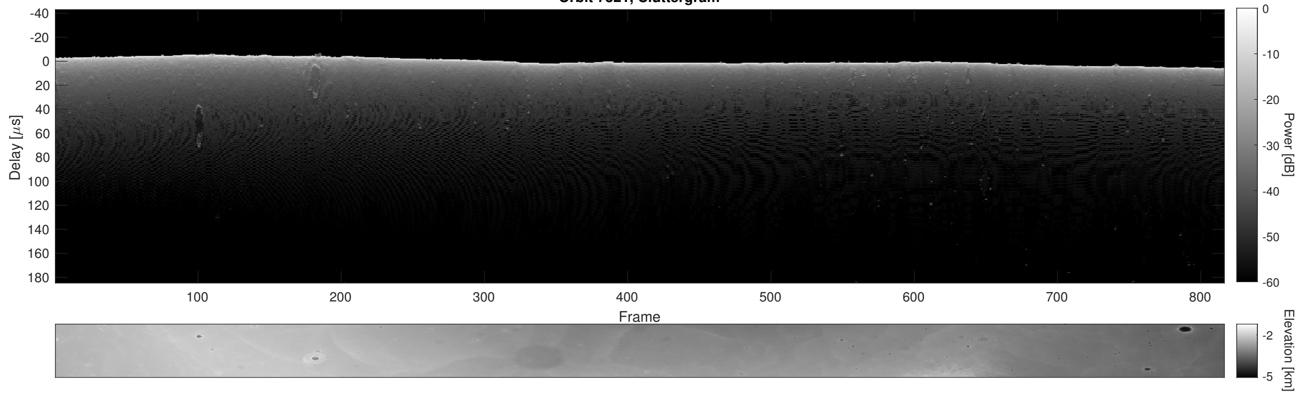
Orbit 7321, Cluttergram
