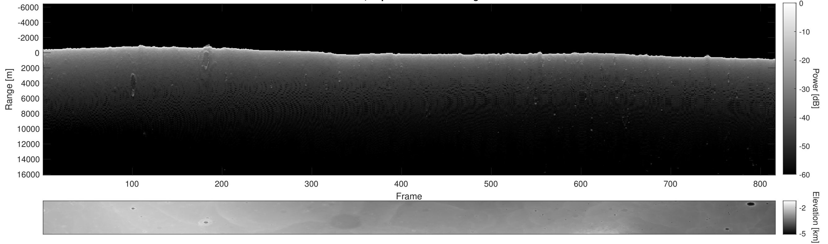
Orbit 7321, Depth-Corrected Cluttergram
