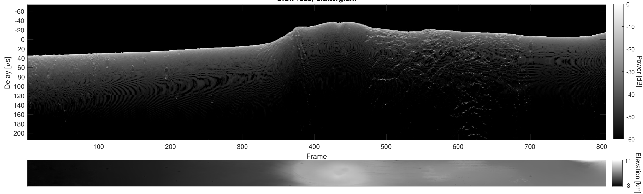
Orbit 7323, Cluttergram
