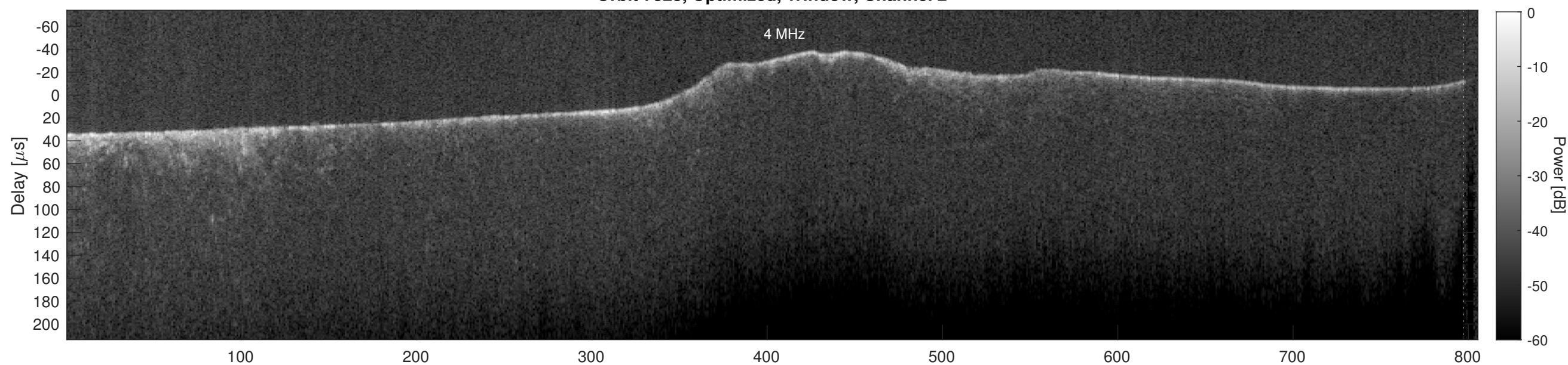
Orbit 7323, Cluttergram
